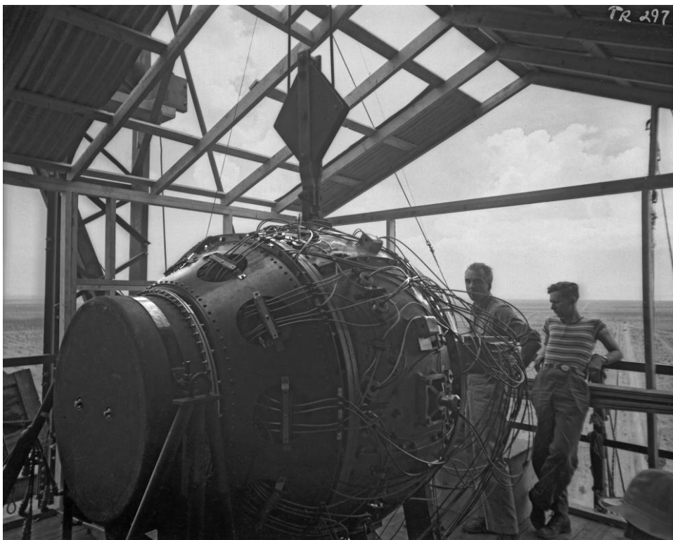
Figure 4. The “Trinity” gadget detonated on 16 July 1945. The detonating switches are in the X-Unit firing device at the front of the bomb. Note the harness and the cables emanating from it. Source: Los Alamos National Laboratory, photo TR-297, part of collection LA-UR-06-1005.
